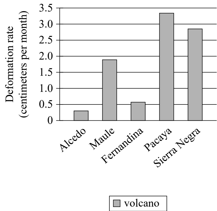
Deformation Rate of Five Volcanoes
